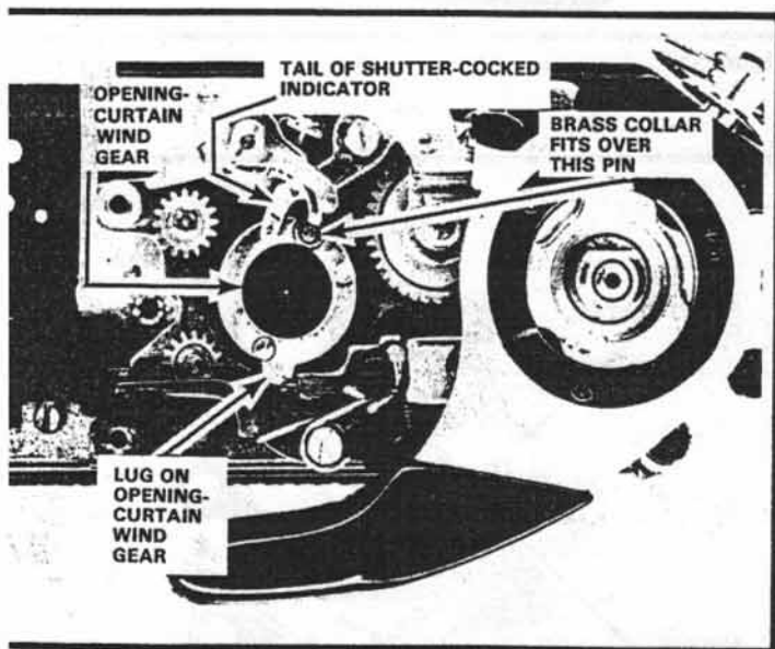
Figure 121 Shutter released
